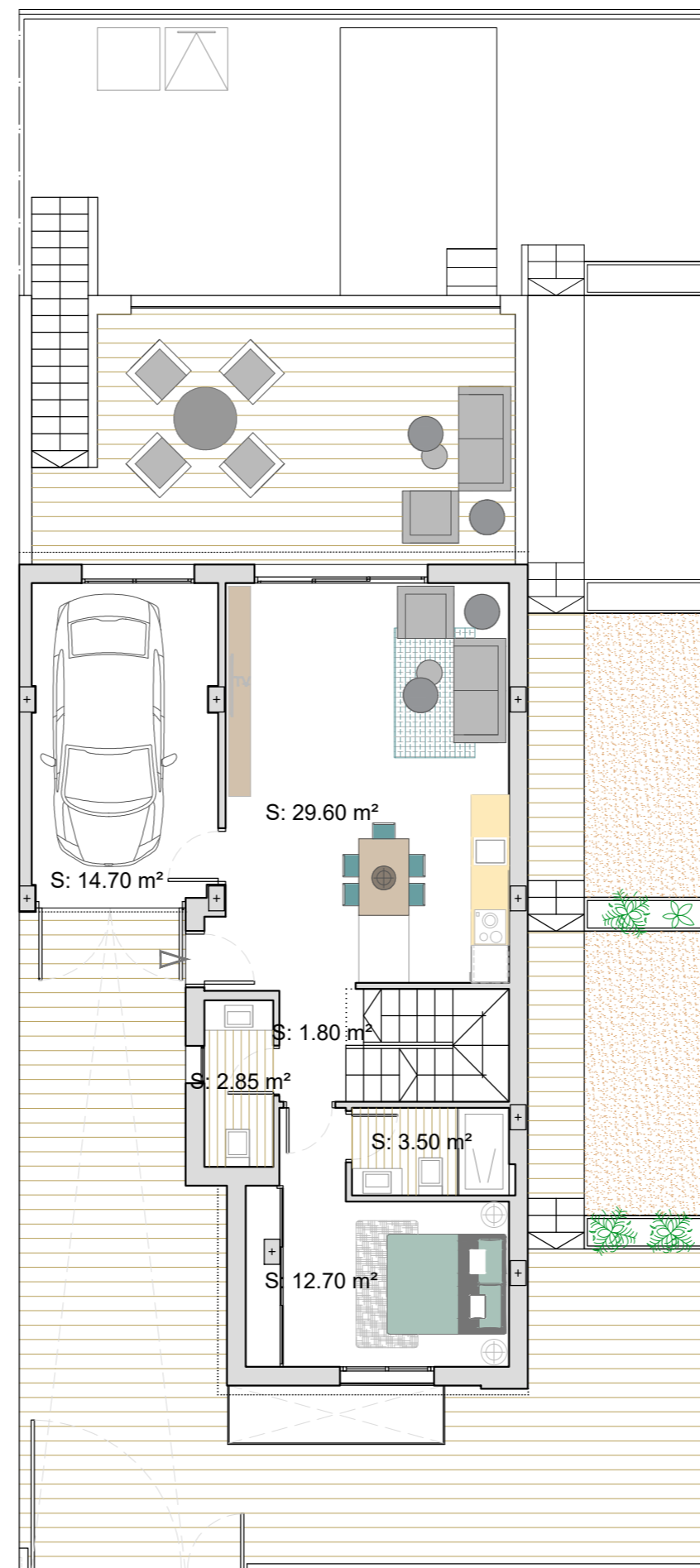
GROUND FLOOR
