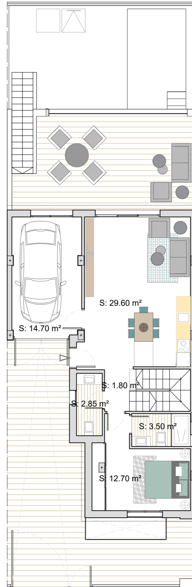
GROUND FLOOR
