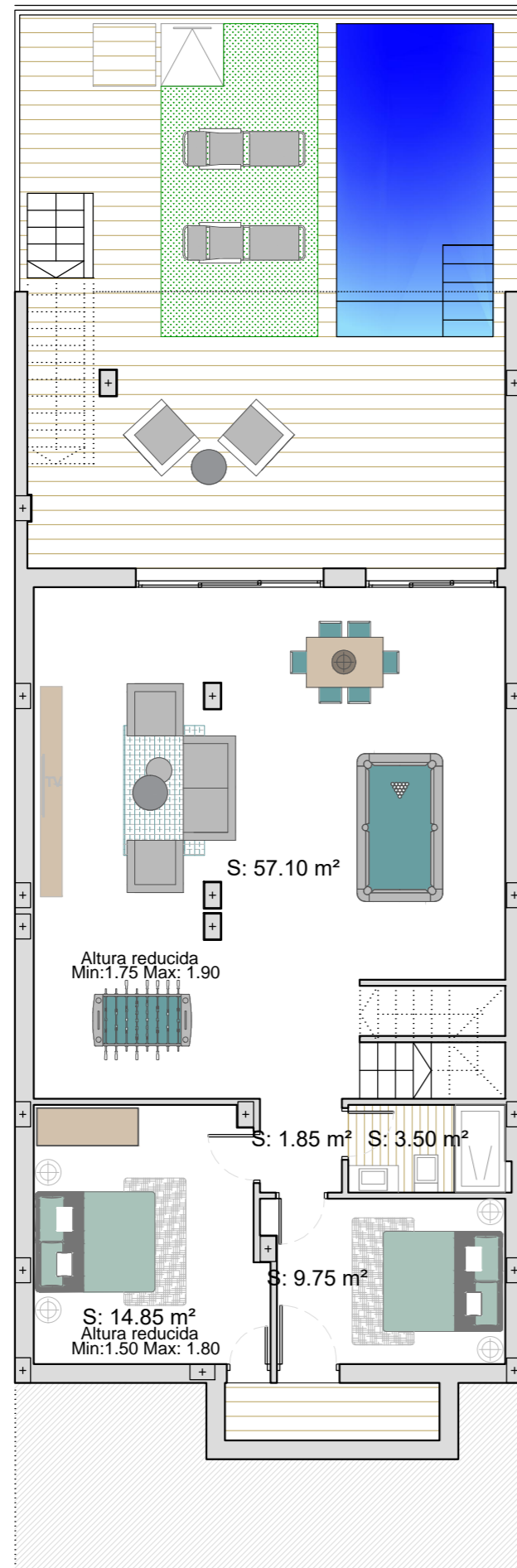
BASEMENT
